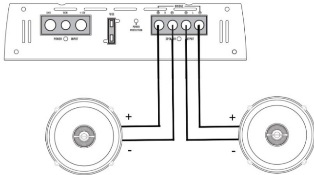
Blaupunkt Speaker wired to a single channel Total Impedance: 4 ohms x channel
