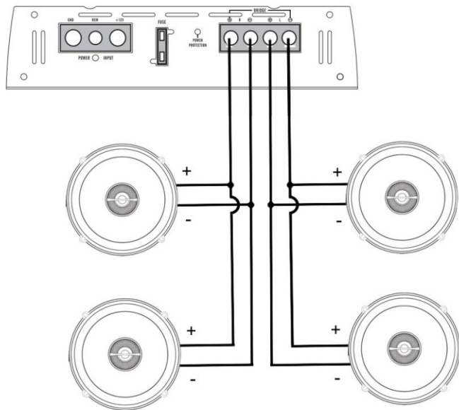
Blaupunkt Speakers wired in parallel to a single channel Total Impedance: 2 ohms x channel
